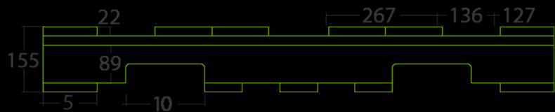
VISTA FRONTAL
